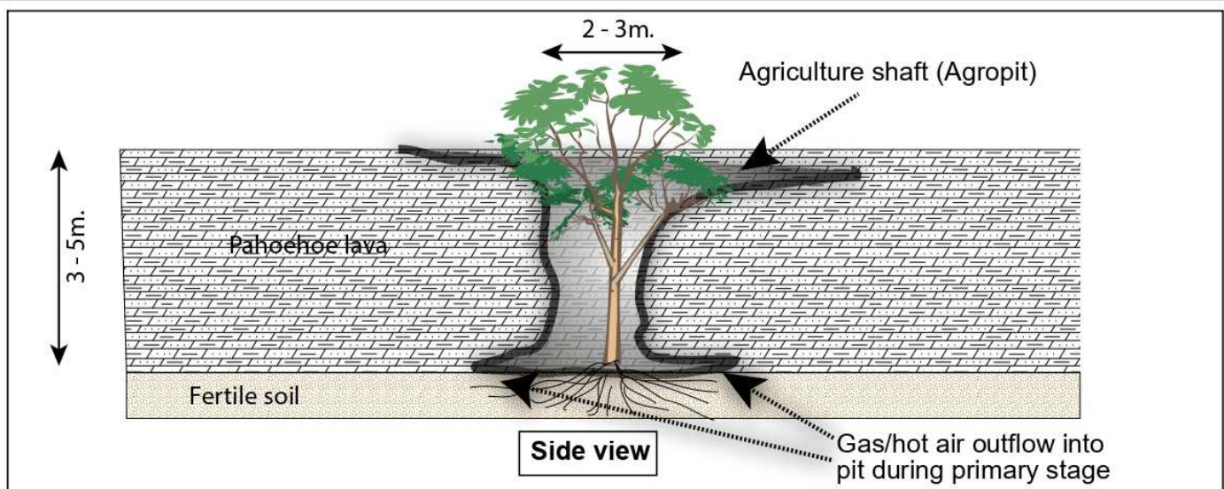
Primary shafts in Pahoehoe lava as shelter for fig trees in Masdache, Lanzarote. Drawing: L. Smets, 07-2023
