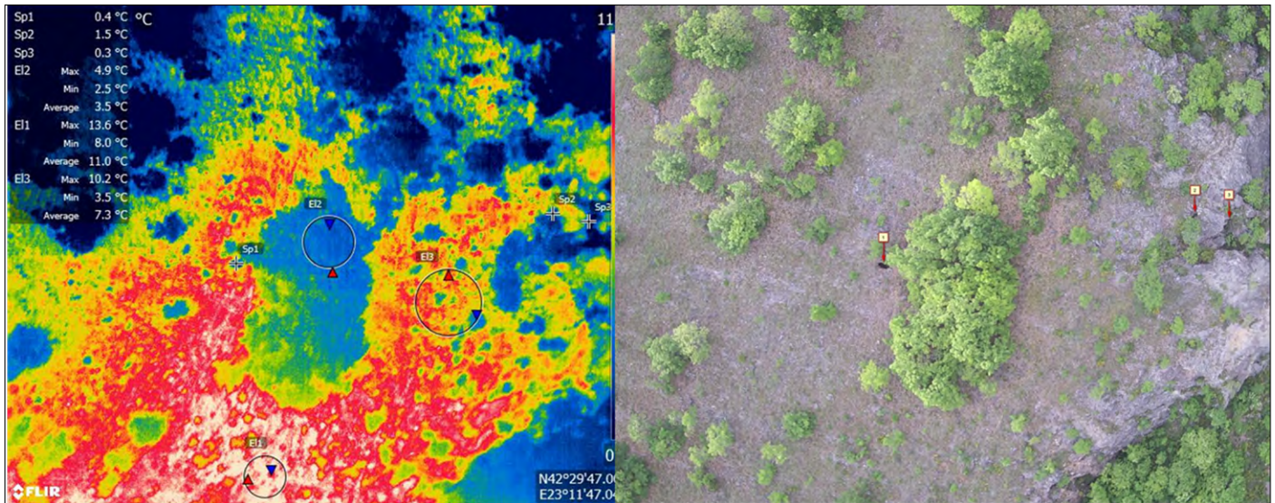
Figure 1: A thermal image of Bosnek Karst taken from a drone from the height of 130 meters with a radiometric thermal camera (left). A shot of the same area from 130 meters high with a visible camera (right). Sp1, Sp2 and Sp3 are unknown cave entrances. Temperatures of the relevant spots and areas of the terrain (upper left) are measured from its thermal image captured by the radiometric thermal camera. Images by Ognian Ognianov.
