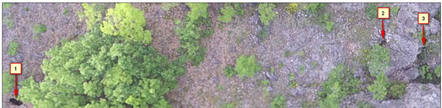
Figure 2: Visible image of the entrances of the three new caves presented on figure 1, taken from a 130 meters high from a UAV. Entrance 1 is located in a vertical section at the edge of the cliff and is therefore not clearly visible in the photograph. Entrance 2 is partially covered with bushes.
